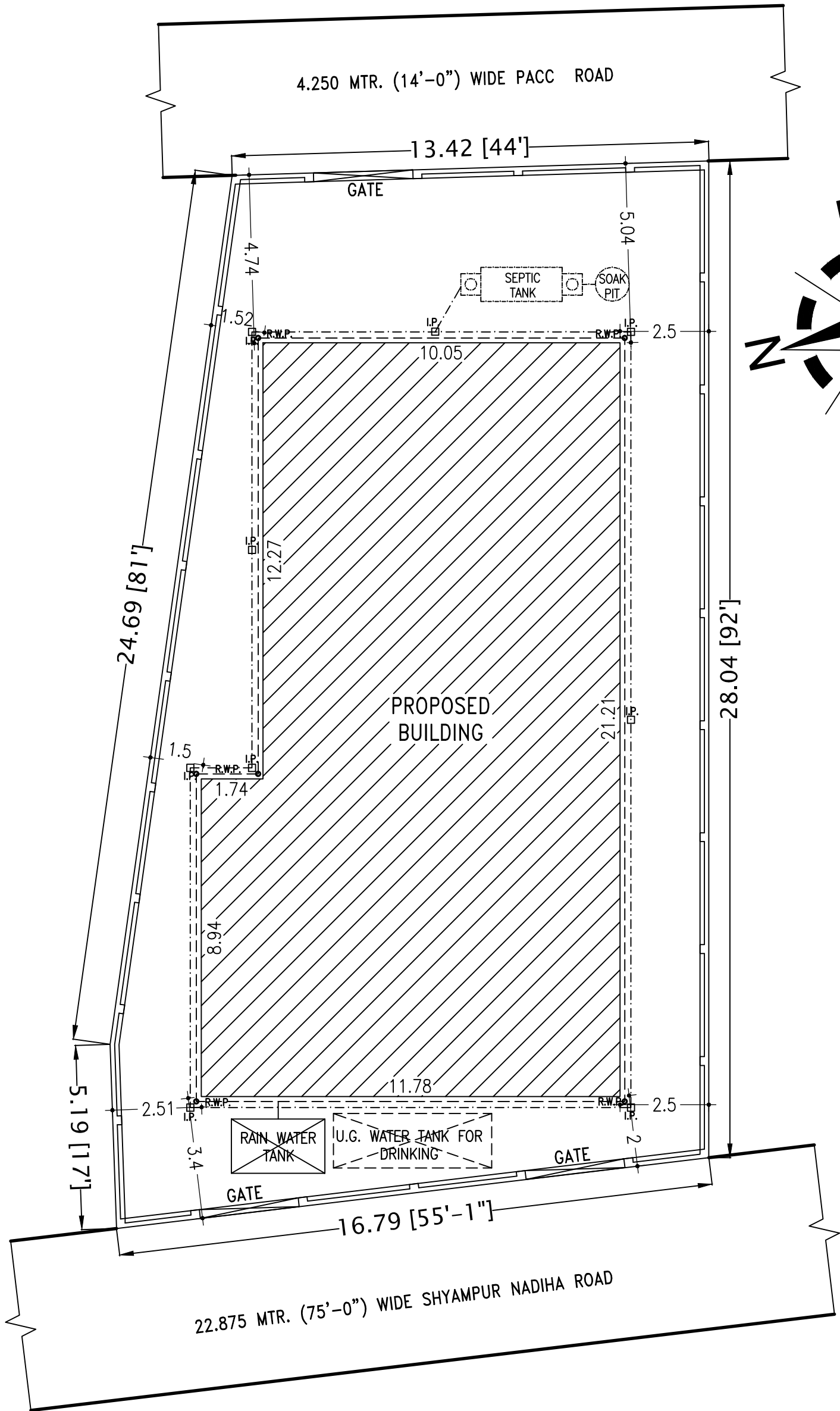
WATER & SEWERAGE PLAN SCALE - 1:200
